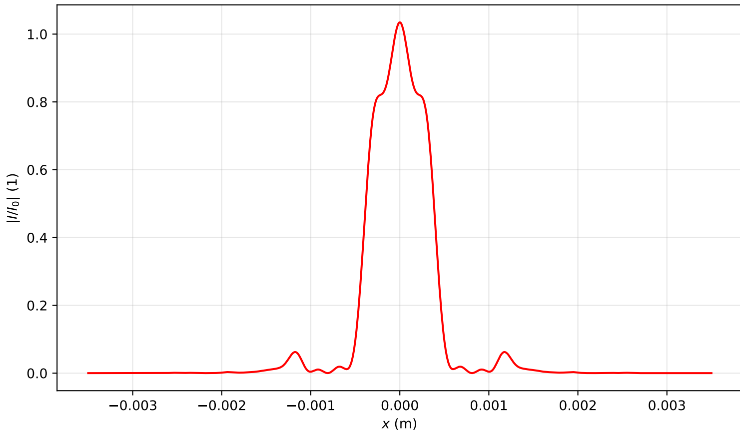
Intensity profile I(x, y = 0, z = 1.672)/I_0 , P_{in}=4.0P_{cr} , artificial time
